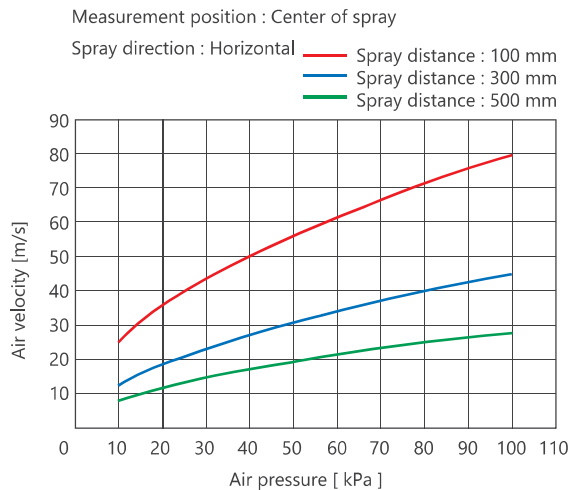
Air velocity characteristics
