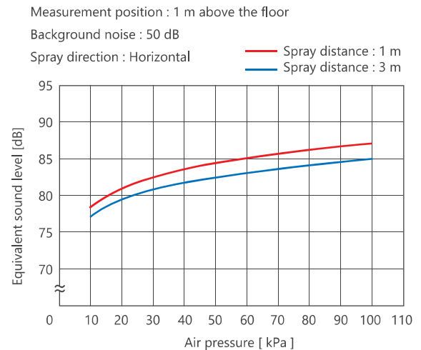
Noise level characteristics
